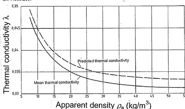
Figure B.2 — Relationship between declared thermal conductivity (at 50 mm reference thickness) and apparent density; 1 - \alpha = 0,90 ; n = 3873
