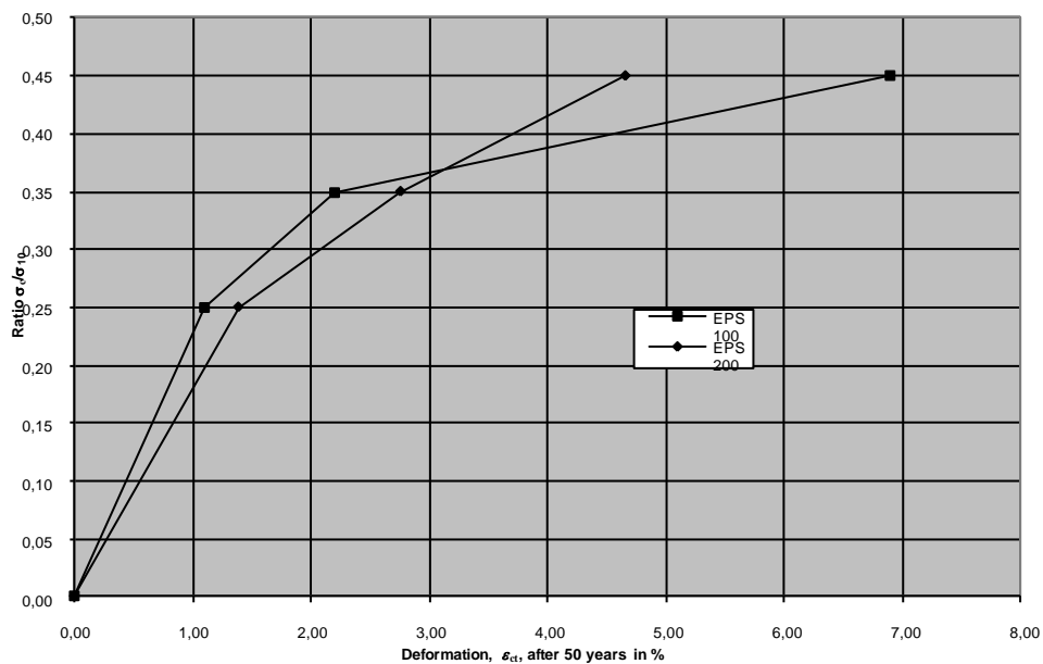
Figure 11: Measured total deformation of EPS 200, \varepsilon_t , and extrapolation to 50 years.
