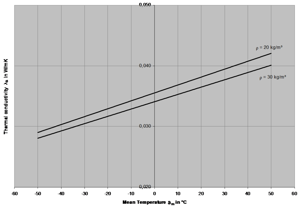
Figure 2: Thermal conductivity of EPS versus mean temperature derived from reference [20].
