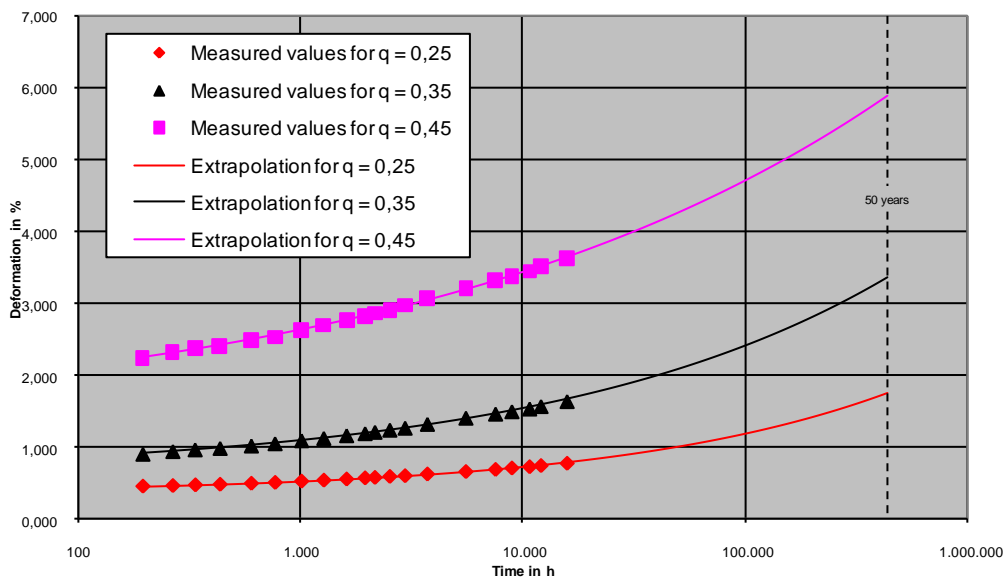
Figure 11: Measured total deformation of EPS 200, \varepsilon_t , and extrapolation to 50 years.
