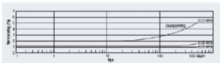
Figure 4: Time/deformation curve of EPS 150
