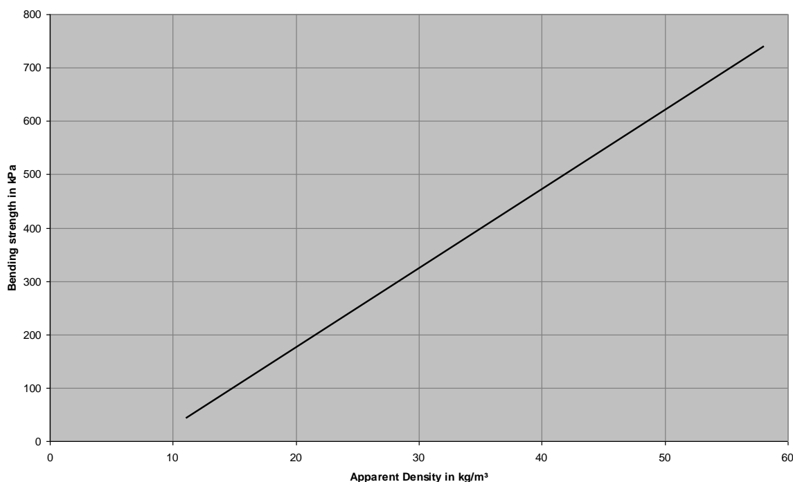
Figure 4: Correlation between bending strength and density.
