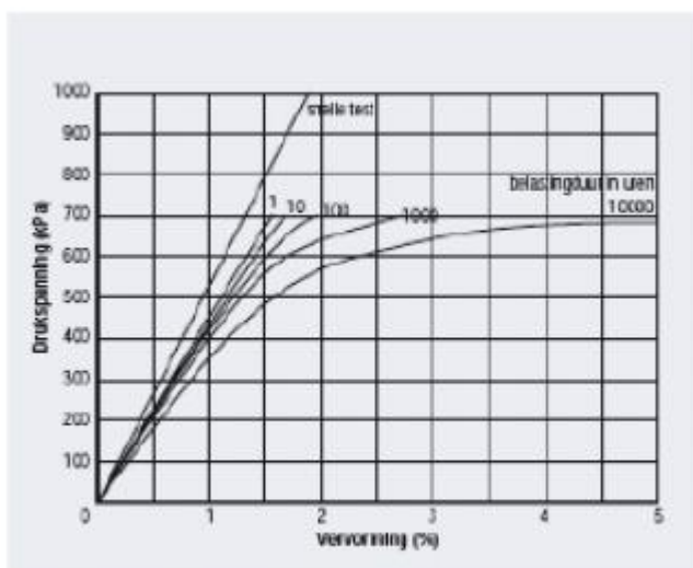
Figure 5: Stress/deformation diagram at various times
