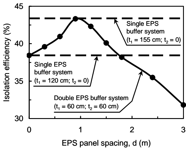
Fig. 6. Seismic isolation efficiency in relation to the EPS panel spacing for double EPS geofoam buffer system with individual EPS panel thicknesses t_1 = t_2 = 60 cm.
