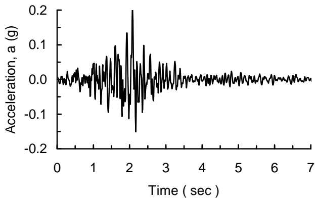
Fig. 3. Input horizontal seismic excitation.
