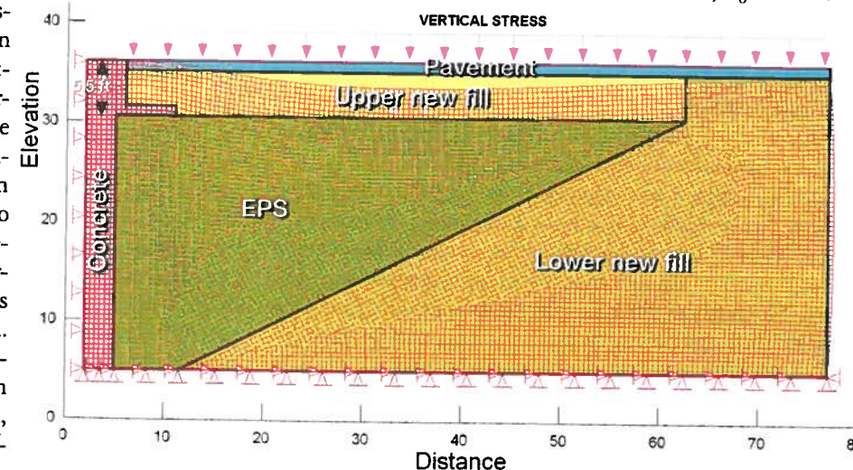
SAMPLE ESTIMATED DEFORMATION OF THE EPS
