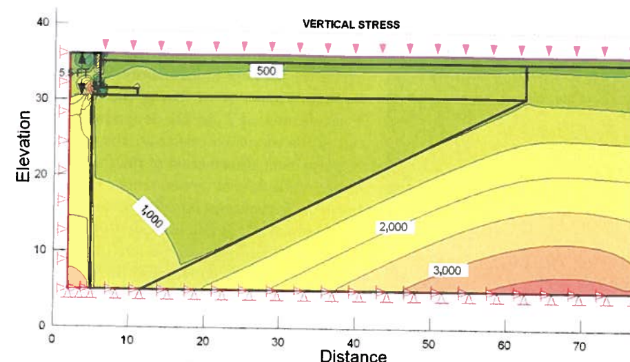
SAMPLE VERTICAL STRESS DISTRIBUTION THROUGH EPS AND CONVENTIONAL FILL AND LOAD TRANSFER TO EXISTING BUILDING
