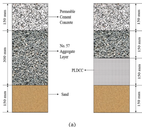
Fig. 4. Infiltration test: (a) schematic diagrams of the permeable paving with and without PLDCC; (b) the laboratory sections.
