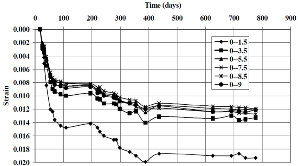
Figure 1.5 Construction and Postconstruction Strain in EPS
