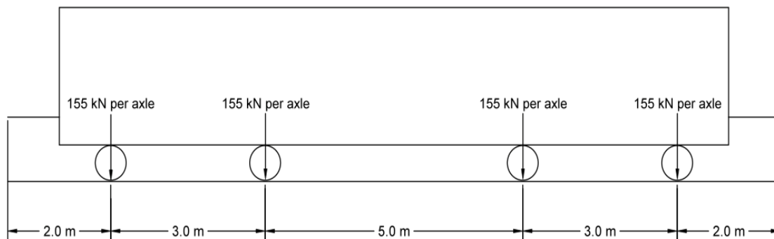
Figure 4.13 Loading Conditions
