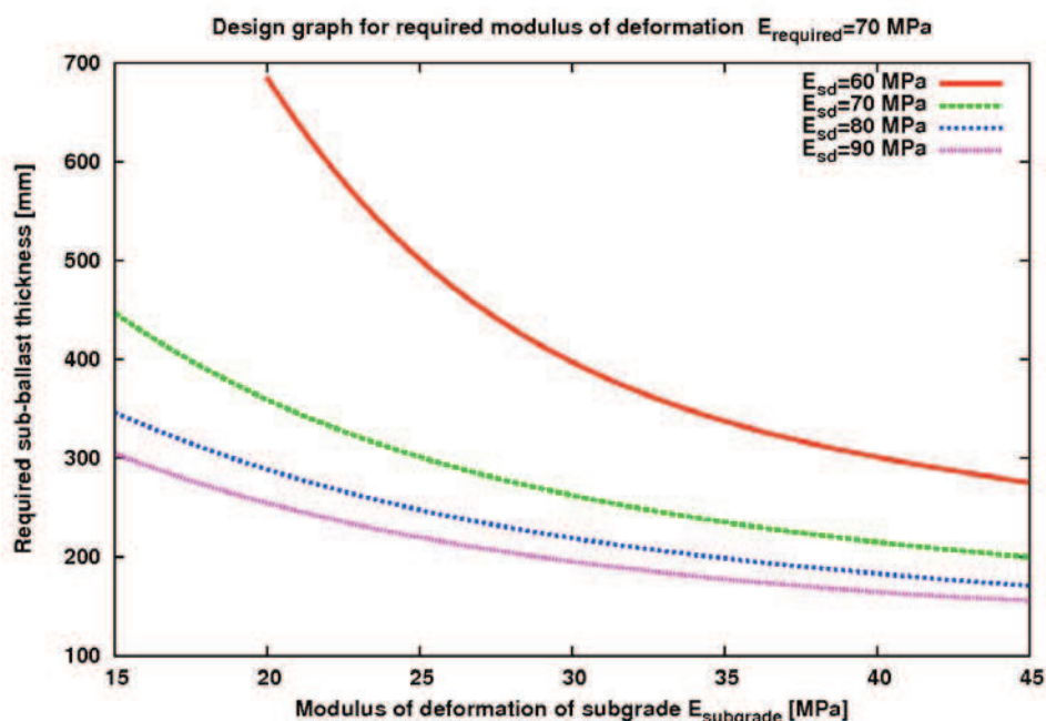
Fig. 9 Design graph for required modulus of deformation E=70 \text{ MPa} , thickness of the top ballast layer 250 mm
