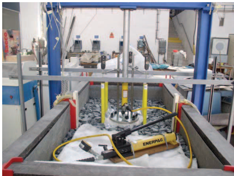
Fig. 4 Static plate load test
