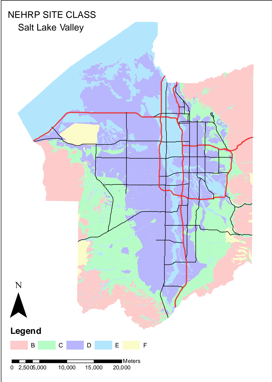
Figure 6. NEHRP Site Class Map for Salt Lake Valley, Utah.
