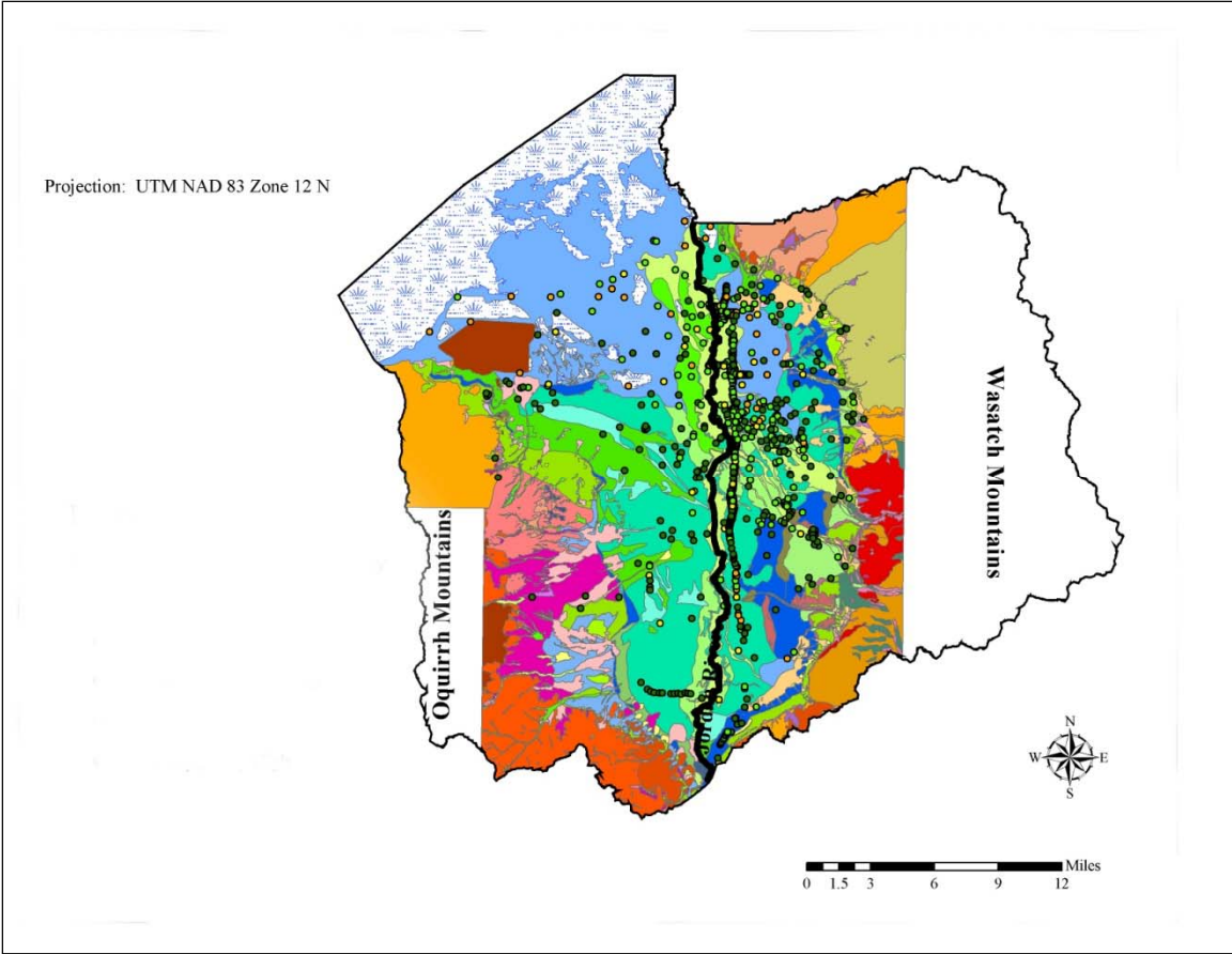
Figure 1. Surficial geologic map and SPT borehole locations.
